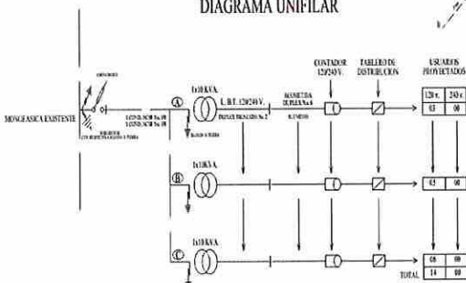
DIAGRAMA UNIFILAR
